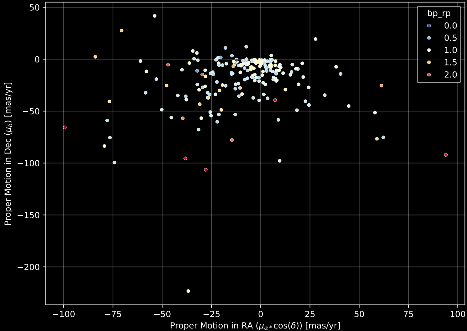
APOGEE DR17 Field: [190+44_MGA] Proper Motion Diagram (n= 200)
