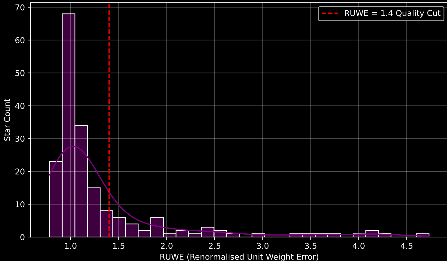
GAPOGEE DR17 Field [190+44_MGA] RUWE Distribution (n= 186)
