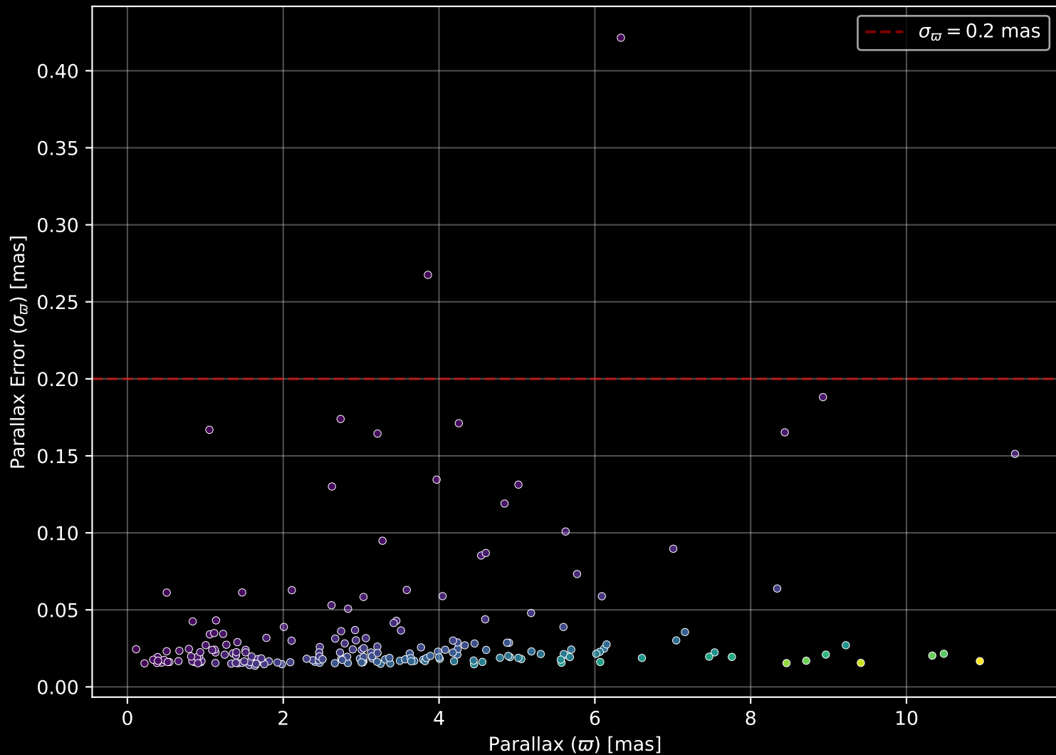
APOGEE DR17 Field: [190+44_MGA] Parallax Quality (n= 200)
