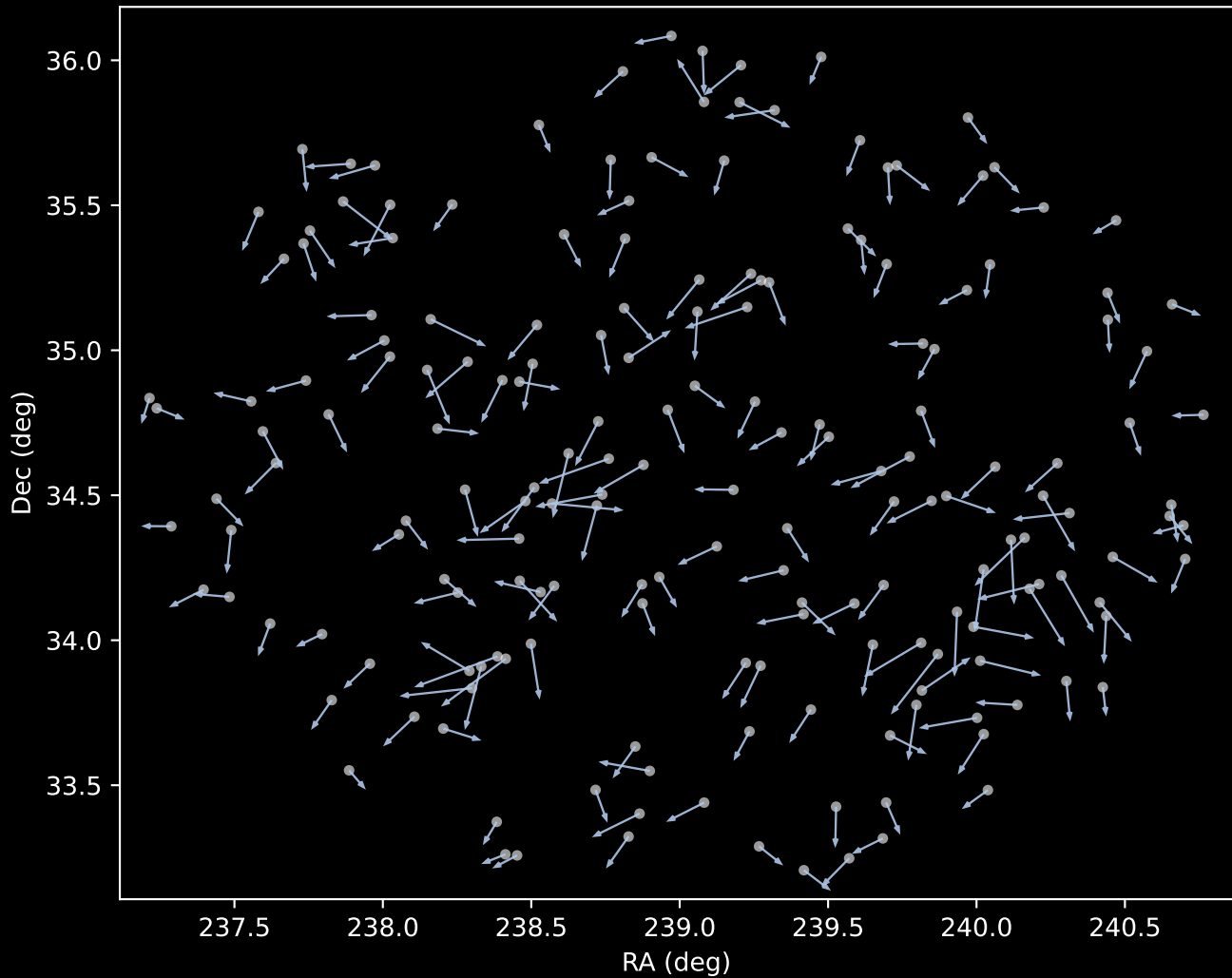
APOGEE DR17 Cluster 1 Proper Motion Vectors (n=184)
