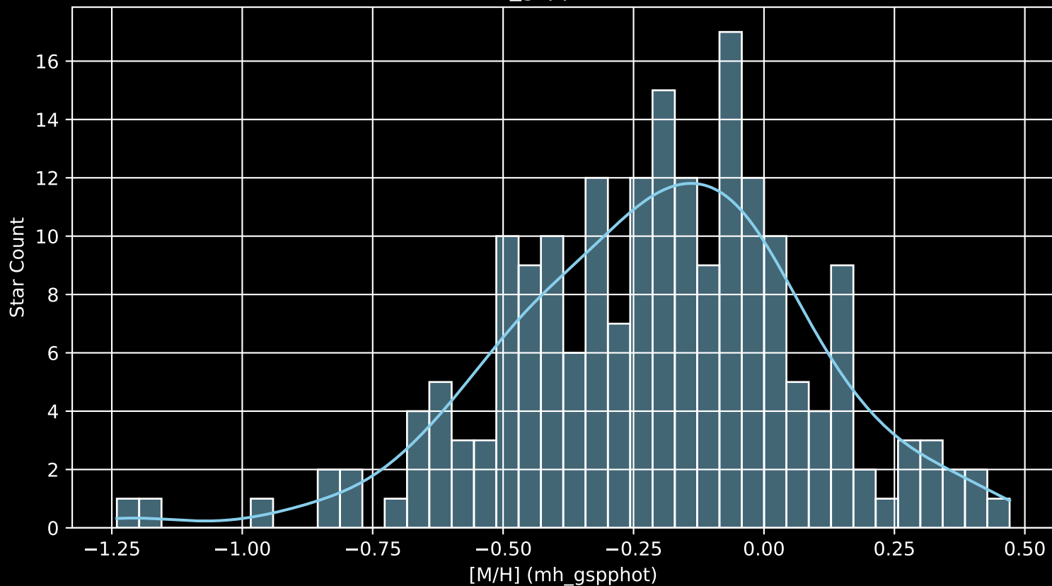
APOGEE DR17 Field: [190+44_MGA [M/H] (mh_gspphot) (n= 196)
