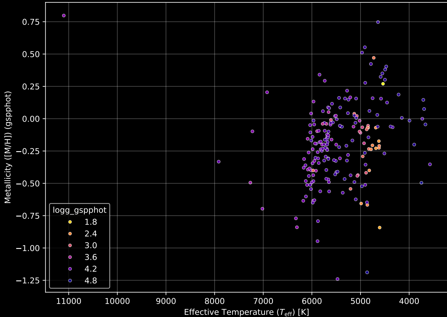
APOGEE DR17 Field: [190+44_MGA] Stellar Population Parameters (n= 200)
