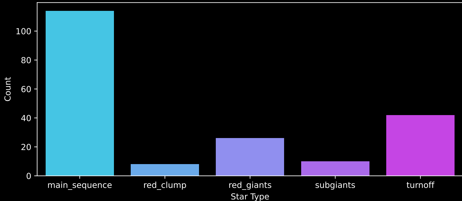
APOGEE DR17 Field: [190+44_MGA] Count plot of Star Type
